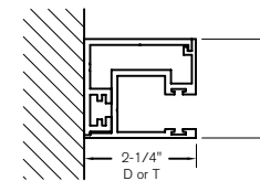
Between Jamb Mount Aluminum & Steel
