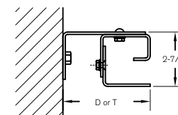
Between Jamb Mount Stainless Steel
