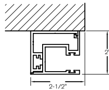
Face of Wall Mount Aluminum & Steel
