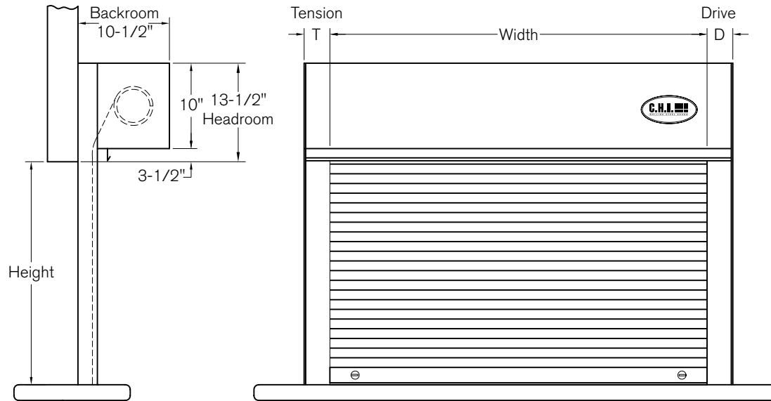
Face of Wall Mount Aluminum & Steel
